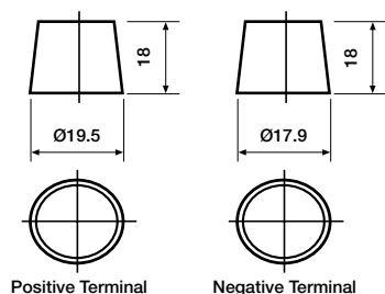
Positive Terminal
