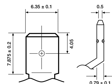
Negative Terminal
